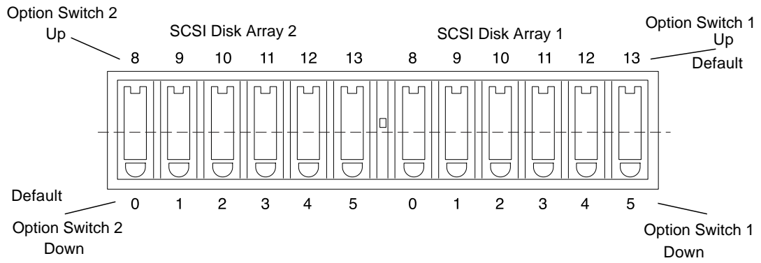
FIGURE 2-7 Sun StorEdge D1000 SCSI Disk ID Address Assignment —12-drive system
